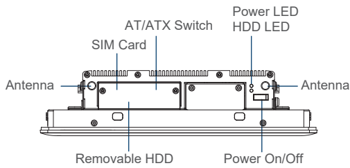
Front I/O
