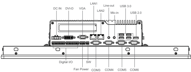
Front I/O
