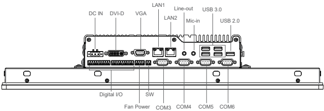
Front I/O
