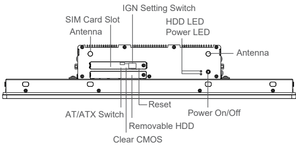
Front I/O
